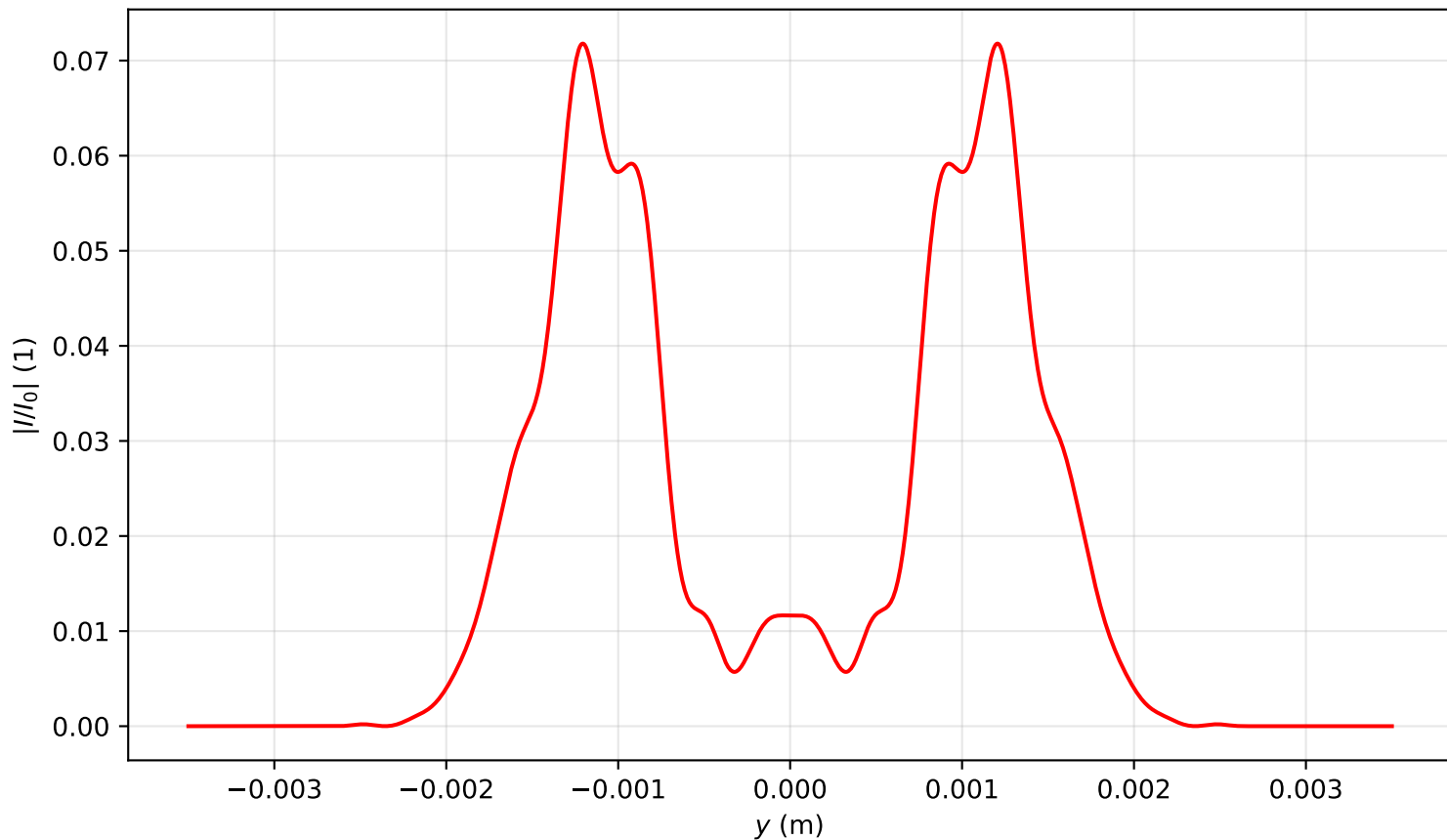
Intensity profile I(x=0, y, z=3.344)/I_0 , P_{in}=6.5P_{cr} , artificial time
